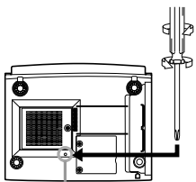
Position selecting screw for ceiling mounting
